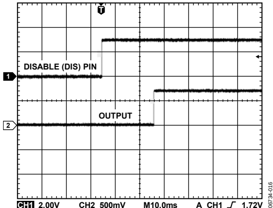
Figure 15. Output Enable
