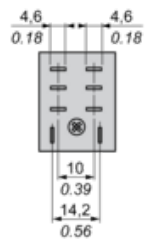
Pin Side View
