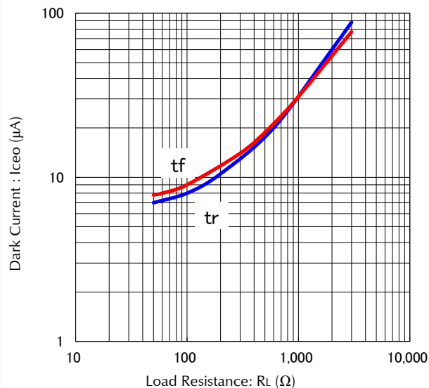
Load Resistance vs. Response Time Condition : V_{ce}=10V , I_c=2mA , T_a=25^\circ C
