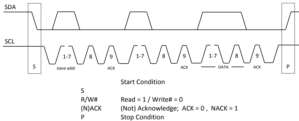
Figure 5: Illustration of voltages during I 2 C communication
