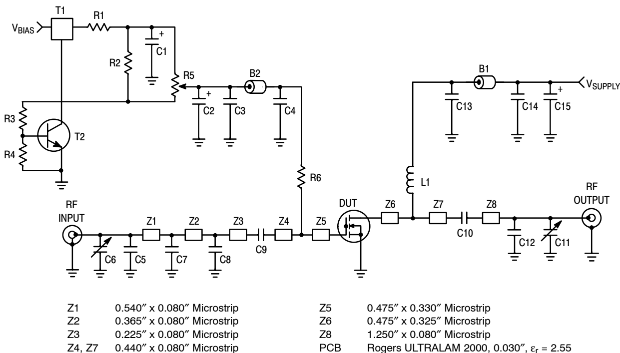
Figure 14. MW6S010MR1(GMR1) Test Circuit Schematic — 450 MHz
