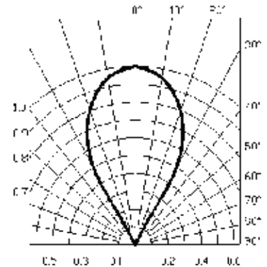
Radiation Diagram
