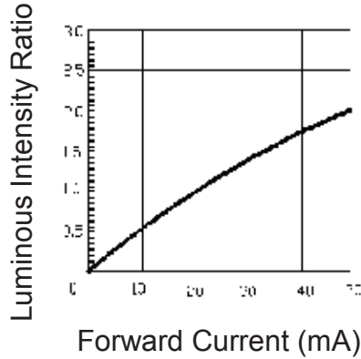
Forward Current vs. Relative Luminous Intensity
