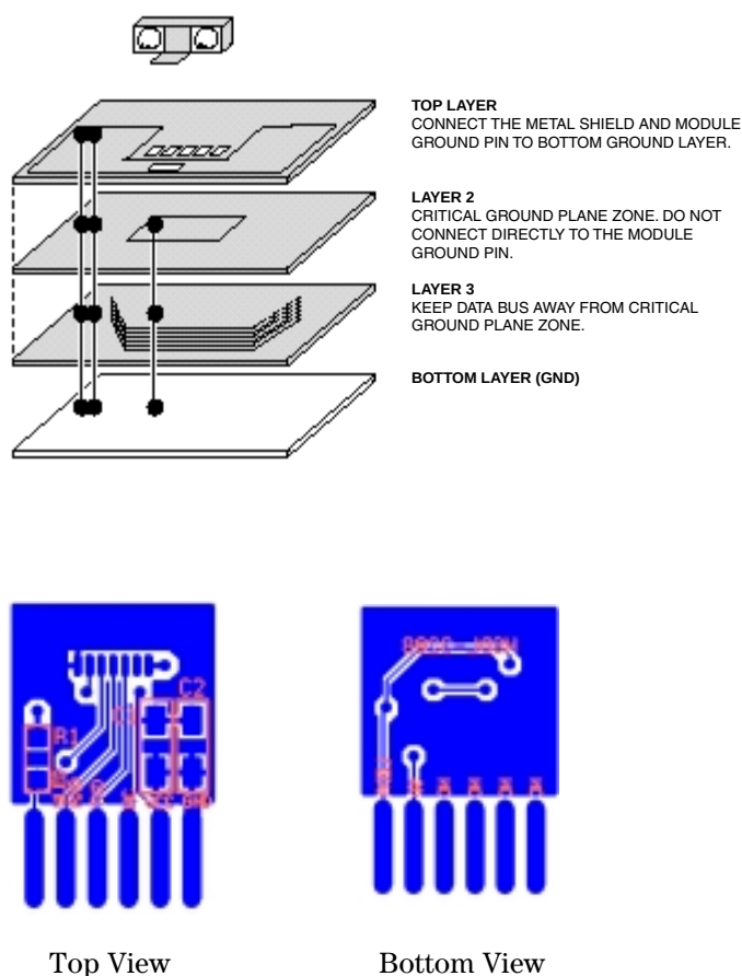
Figure 24. PCB layout suggestion.
