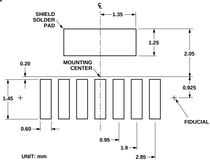
Figure 21. Land Pattern.
