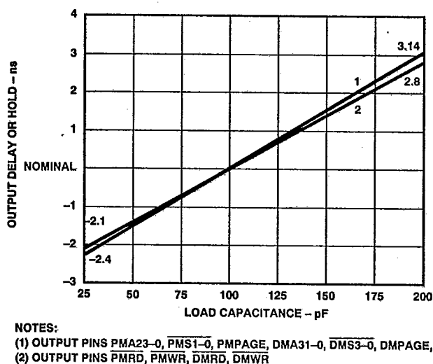
Figure 19. Typical Output Delay or Hold vs. Load Capacitance (at Maximum Case Temperature)
