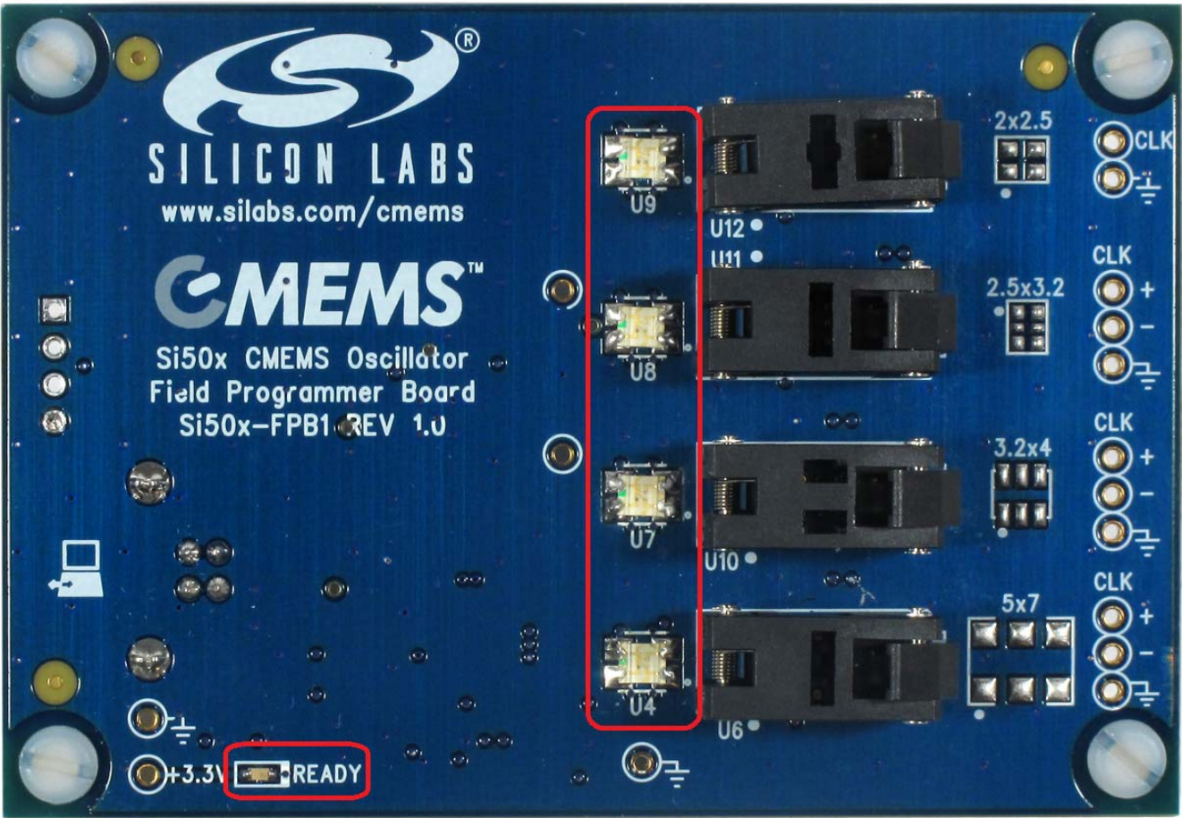
Figure 10. Si501-FPB1 LEDs
