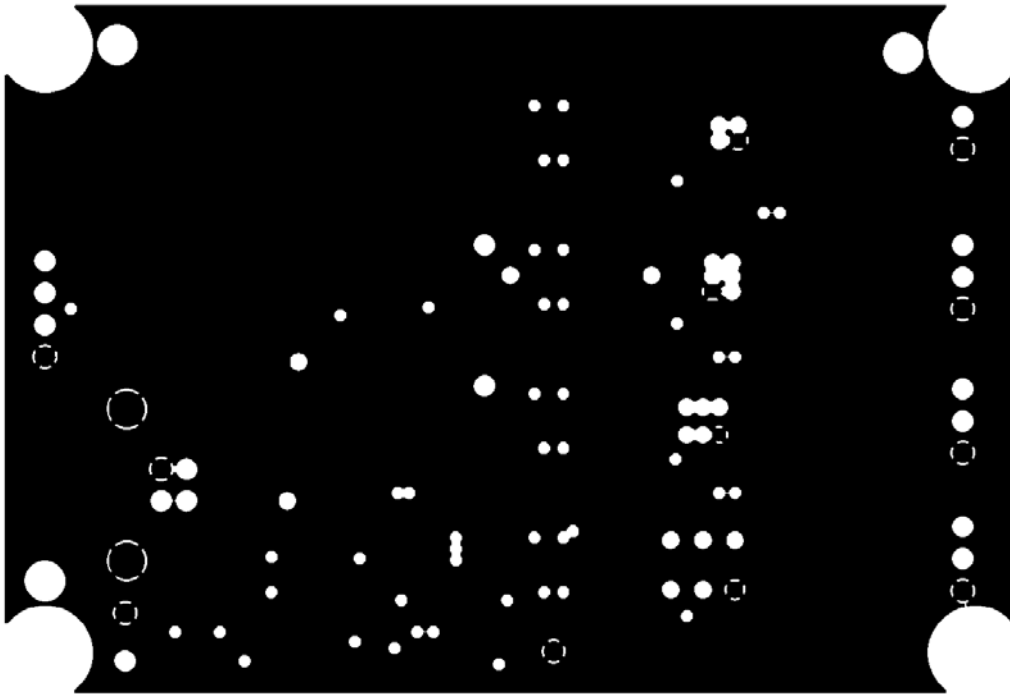
Figure 21. Ground (Layer 3)
