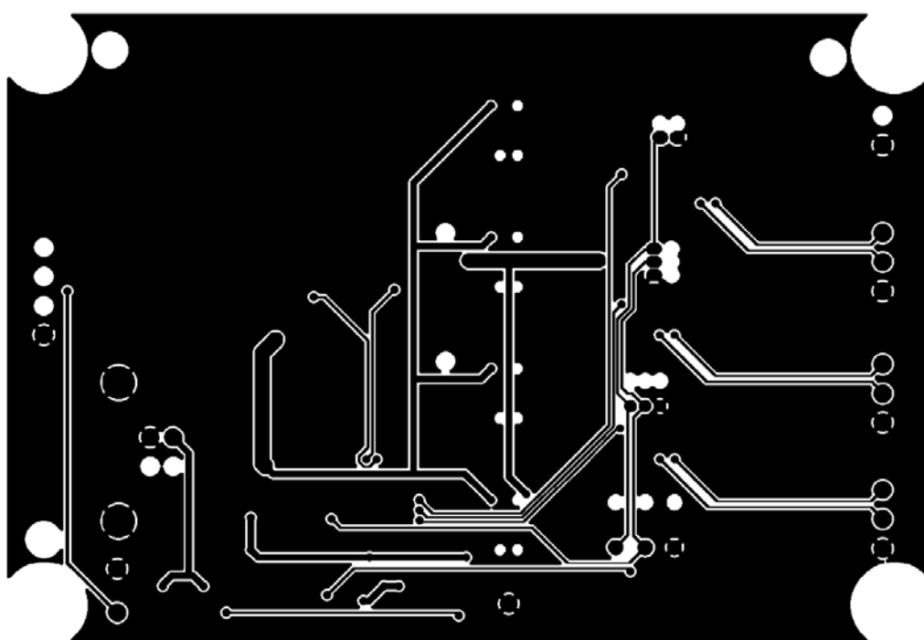
Figure 20. Signal/Ground (Layer 2)
