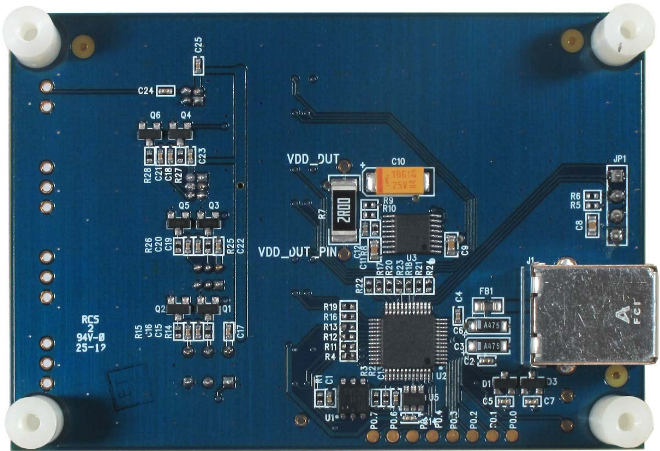
Figure 6. Bottom Board View
