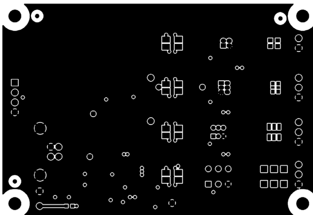
Figure 19. Primary Side (Layer 1)
