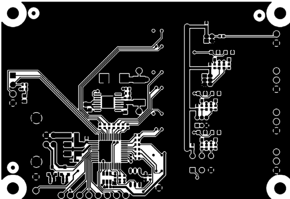
Figure 22. Secondary Side (Layer 4)
