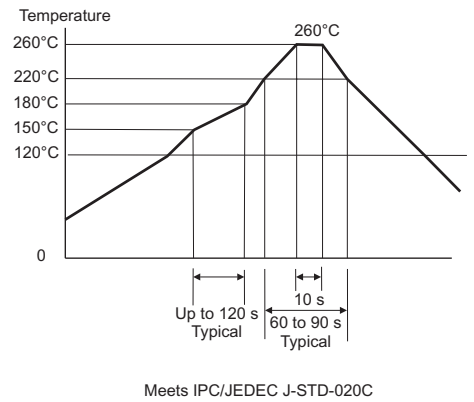
Figure 7: Solder Profile
