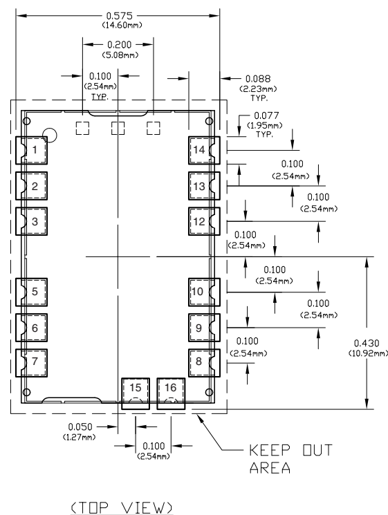
Figure 3: Recommended Pad Layout
