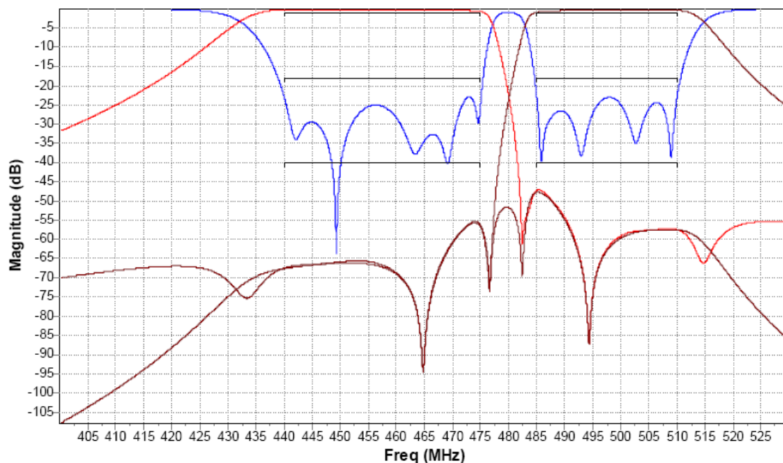
Fig.1 Return Loss and Rejection
