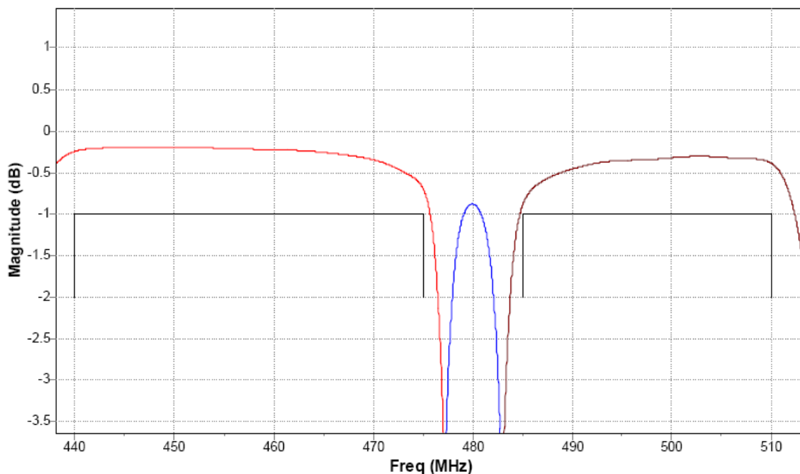
Fig.2 Insertion Loss and Matching
