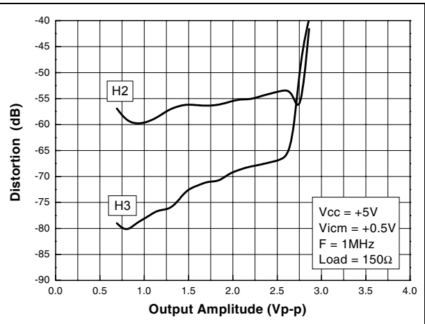
Figure 4. Distortion
